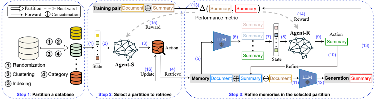
Figure 2: Illustration of M-RAG training in a summarization task: The M-RAG initiates training with multiple partitions (Section 3.1), it then selects a partition to perform retrieval via Agent-S (Section 3.2), and refines the memories within the selected partition via Agent-R (Section 3.3). Both agents are collaboratively trained to enhance generation capabilities through multi-agent reinforcement learning (Section 3.4). For inference, it includes elements (1), (2), (3), (4), (11), and (12).
