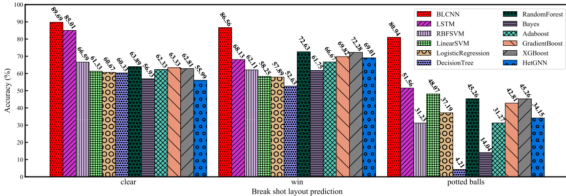
Figure 4: Prediction results.
